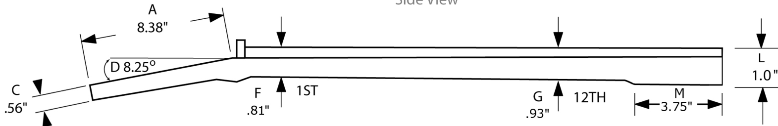
Side View
