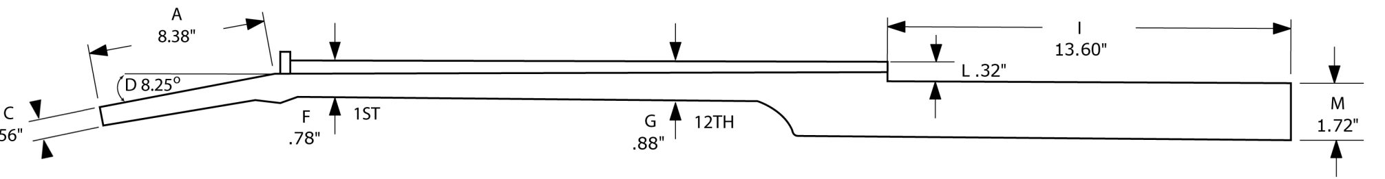
Side View
