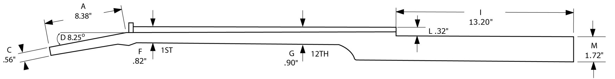
Side View
